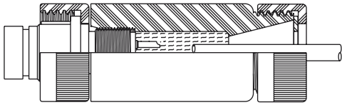
XSL-CCP-FI 45-9
