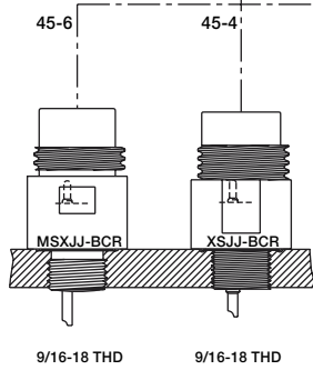
9/16-18 THD
