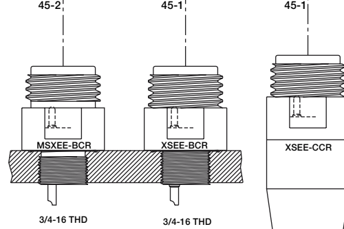
3/4-16 THD
